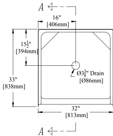
32" [813mm] Shower w/ 8 1/2" [216mm] Threshold & Molded Soap Ledges
